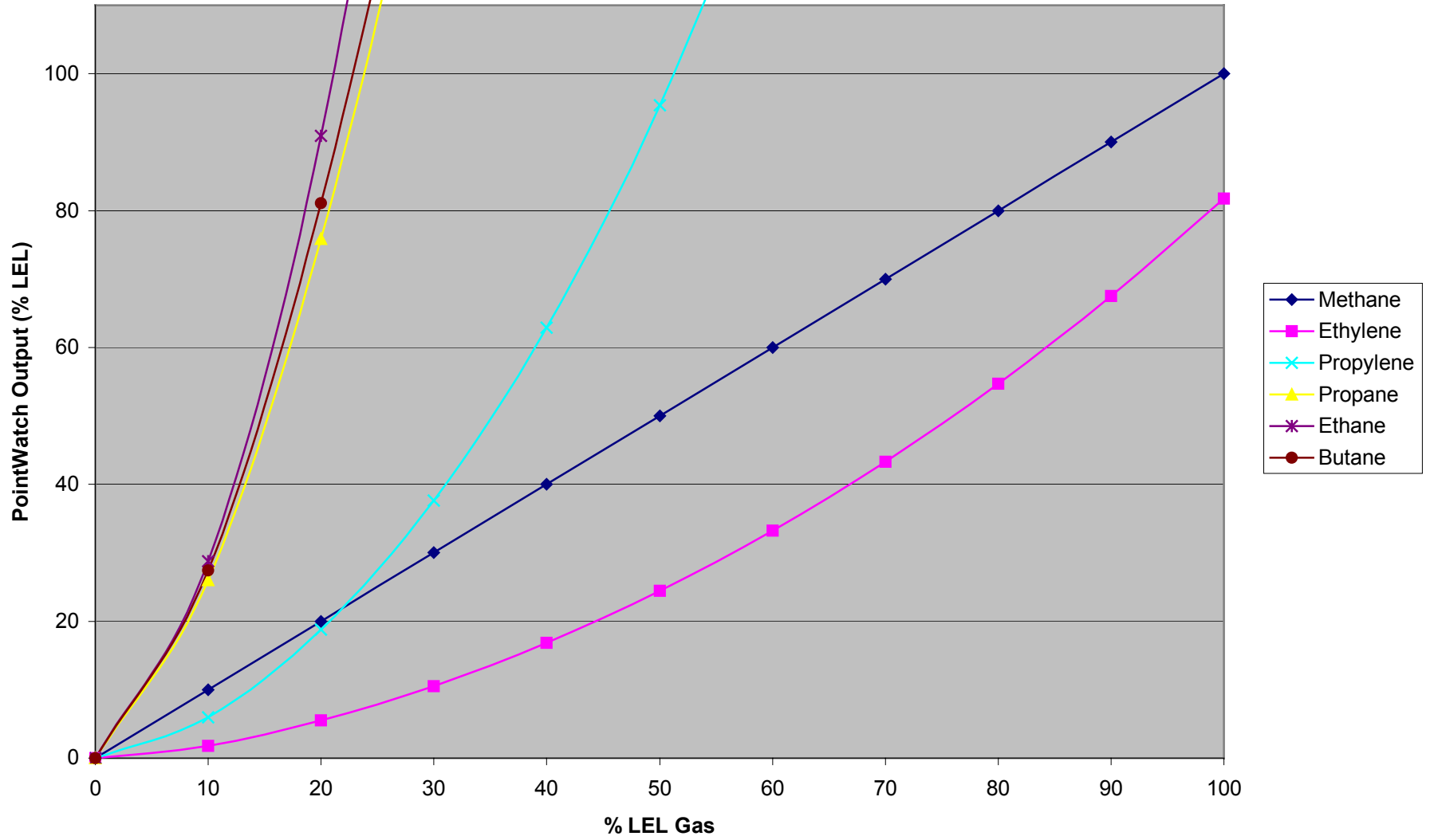
Methane Calibrated PointWatch - Response to Other Gases
